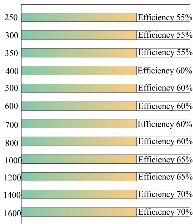
Efficiency of different specification heat exchanger
