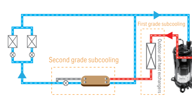
Two-grades subcooling working principle
