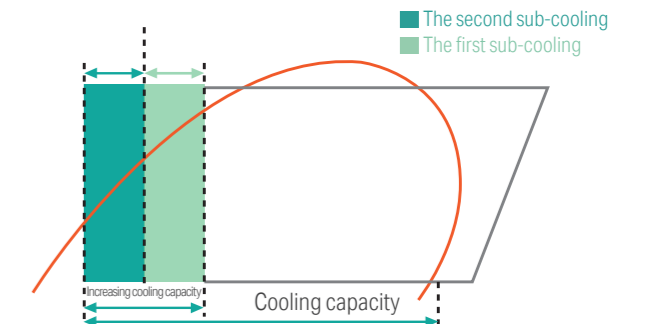
System pressure-enthalpy diagram
