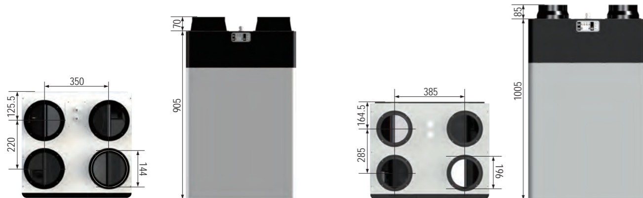
CFA 250T ~ CFA 350T Dimensions
